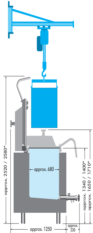
*KA 380 dimensions for gas and oil
